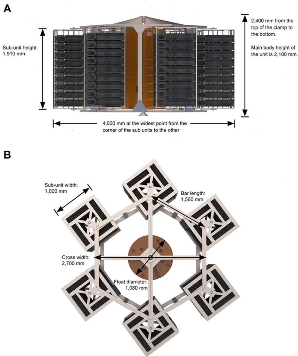
Figure 3: Design and dimensions of the Shellfish Tower™ showing side view (A) and top-down view (B) from Heasman et al., 2021.
